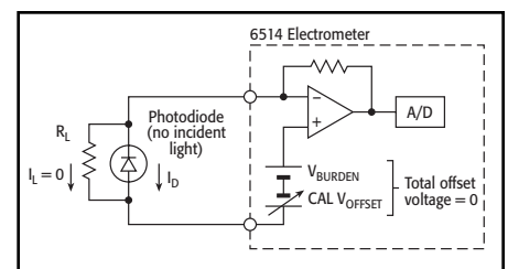
Figure 2. Dark Current Measurement with Burden Voltage Corrected
