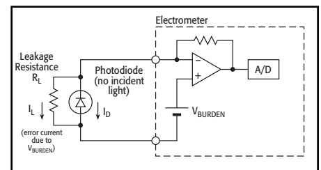
Figure 1. Dark Current Measurement with Burden Voltage Uncorrected
